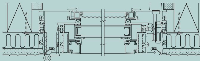
Casement Detail
