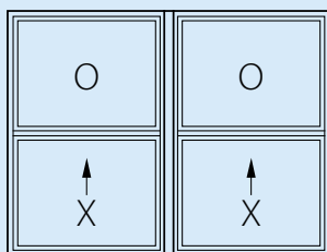
Twin 1/1 by 1/1
